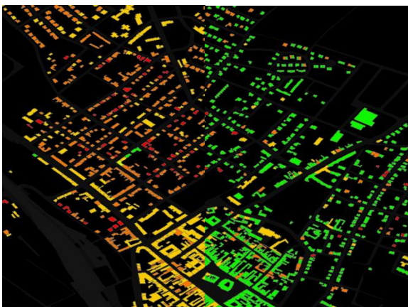
Figure 8: Heating energy demand from green ( < 15 \text{ kWh/m}^2\text{a} ) to red ( > 150 \text{ kWh/m}^2\text{a} ) for the existing building stock (left) and a future city scenario with 80% of the building stock retrofitted to passivhouse standard (right).
